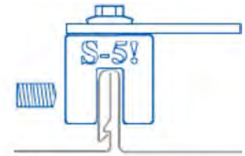
S-Clamp with Adapter Plate
