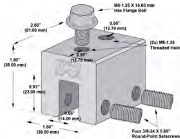
S-5!® S-Clamp
