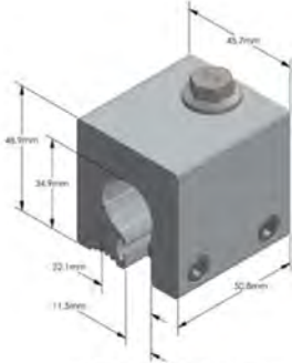
S-5!® Z-Clamp
